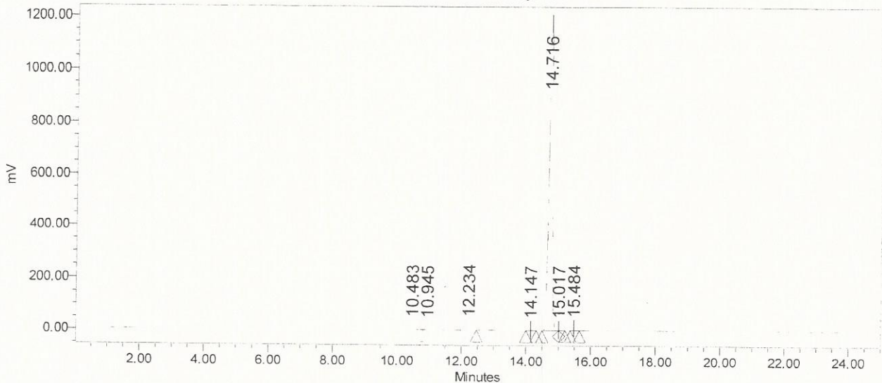
Auto-Scaled Chromatogram
